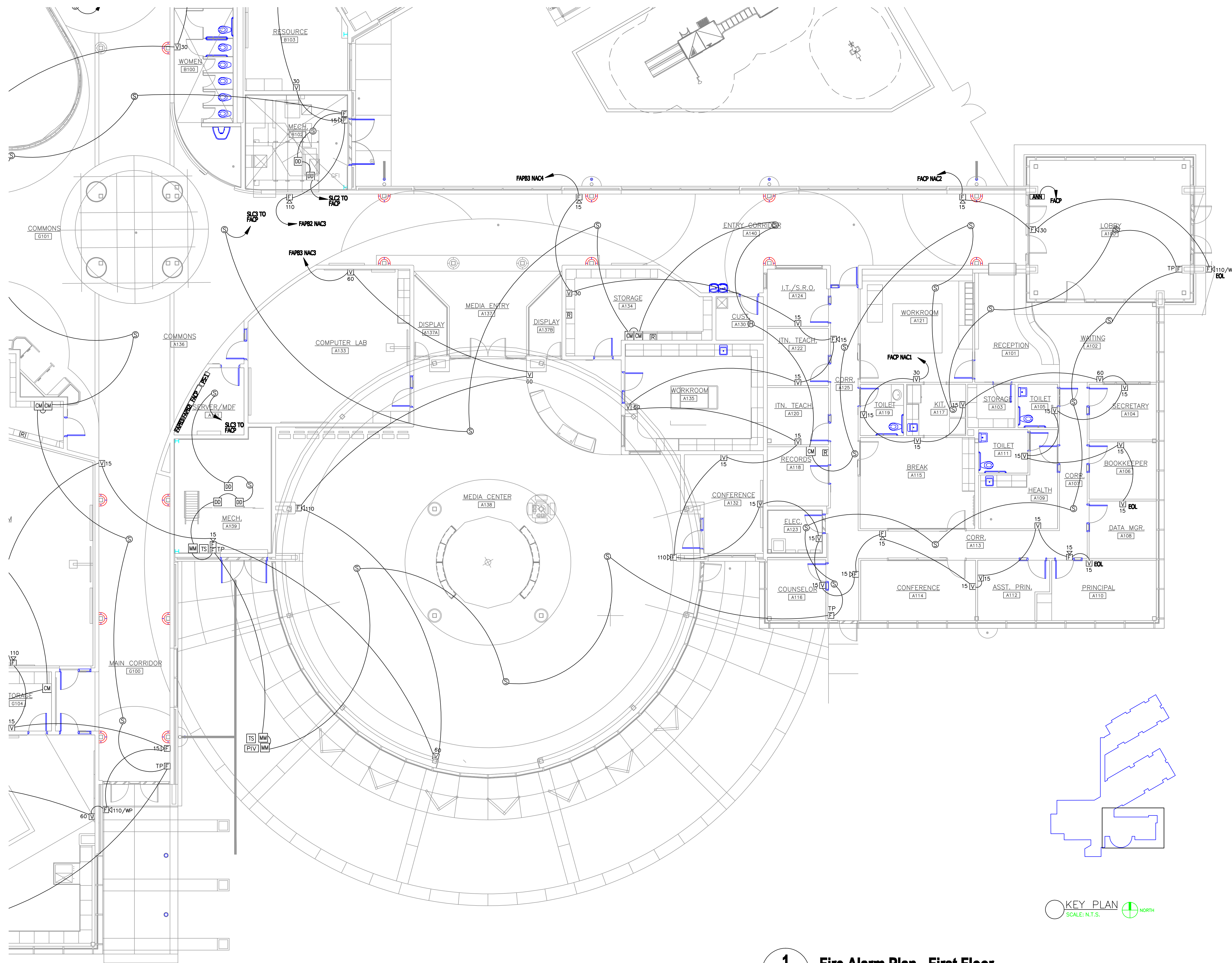
1 FA3 Fire Alarm Plan - First Floor SCALE: 1/8"=1'-0" ADMINISTRATION & MEDIA
